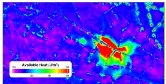
Available heat in place at a 1000m depth for geothermal energy prospecting.
